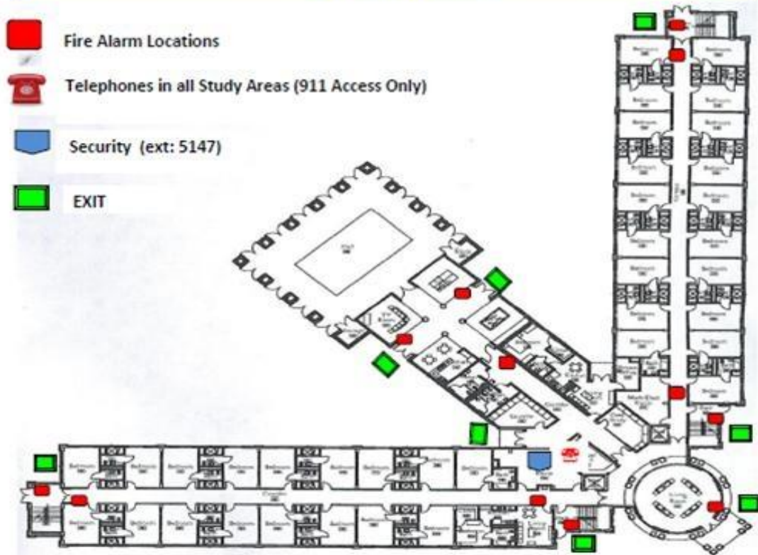
Level One Floor Plan scale: 1" = 30'-0"
